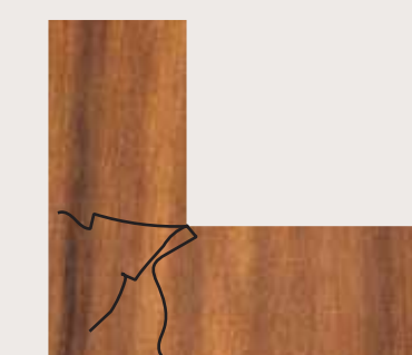
Crack arising due to L shape 90° cutting
