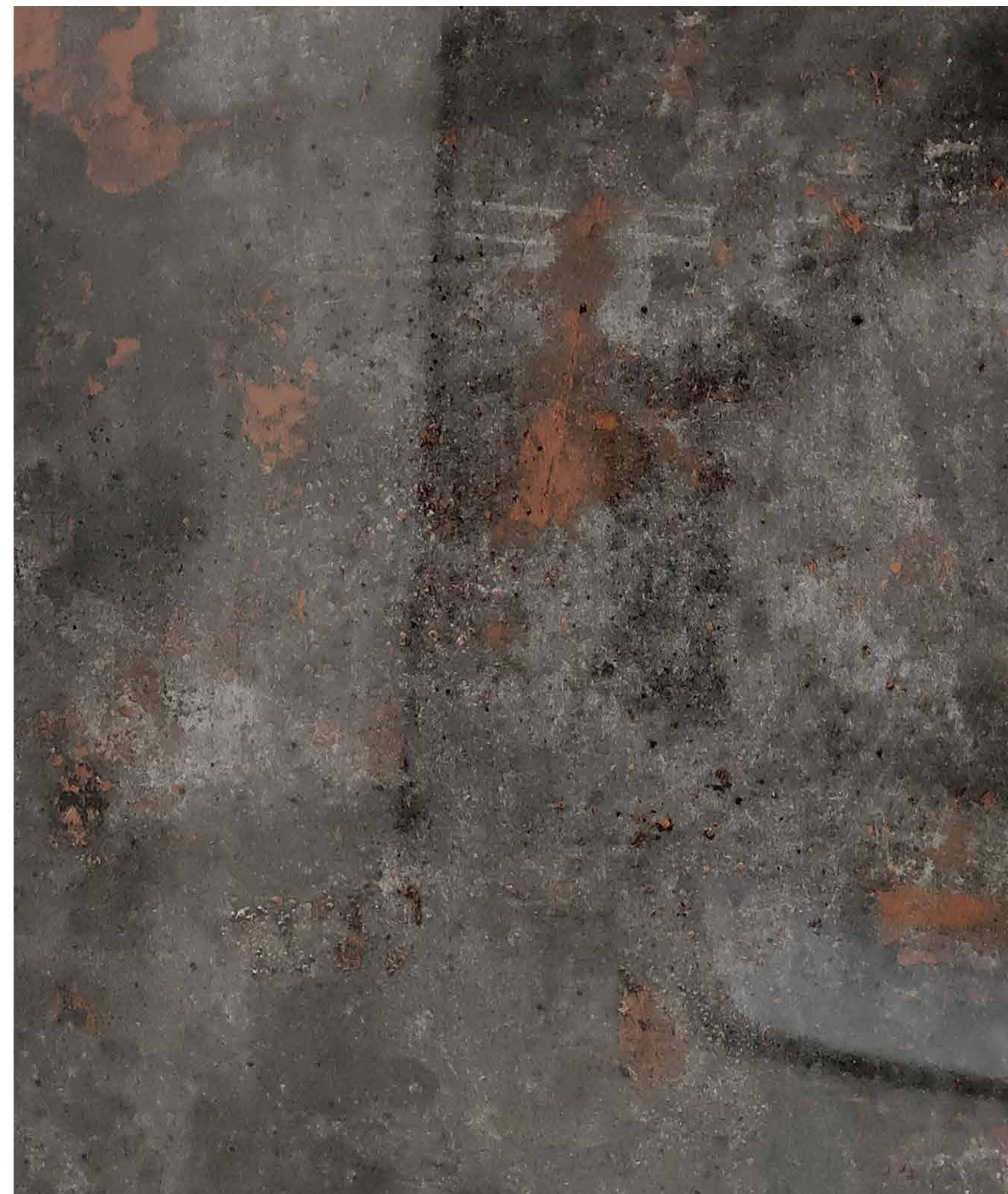
1006 SG | DARK-ICE
