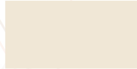
1112 SF | IVORY
