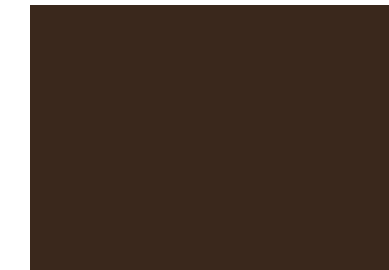
1111 SG | COFFEE
