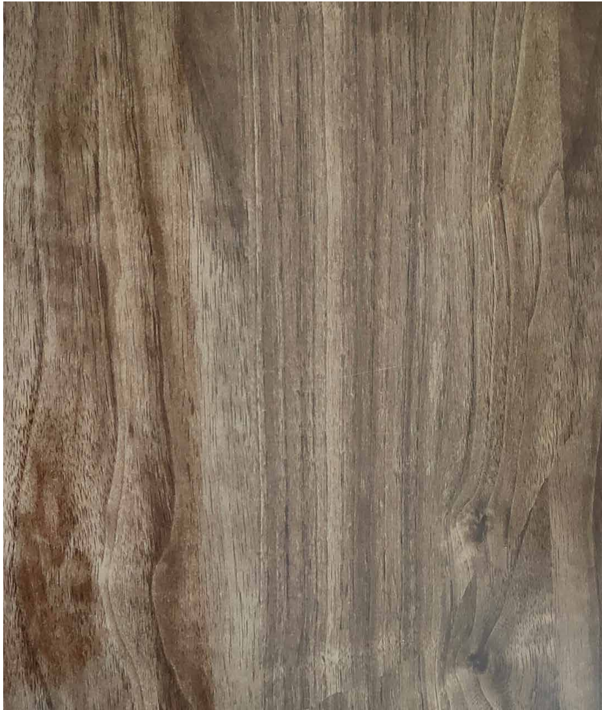
1022 SG | OG-WOOD
