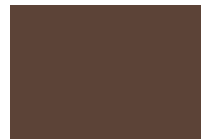
1191 SM | BROWN
