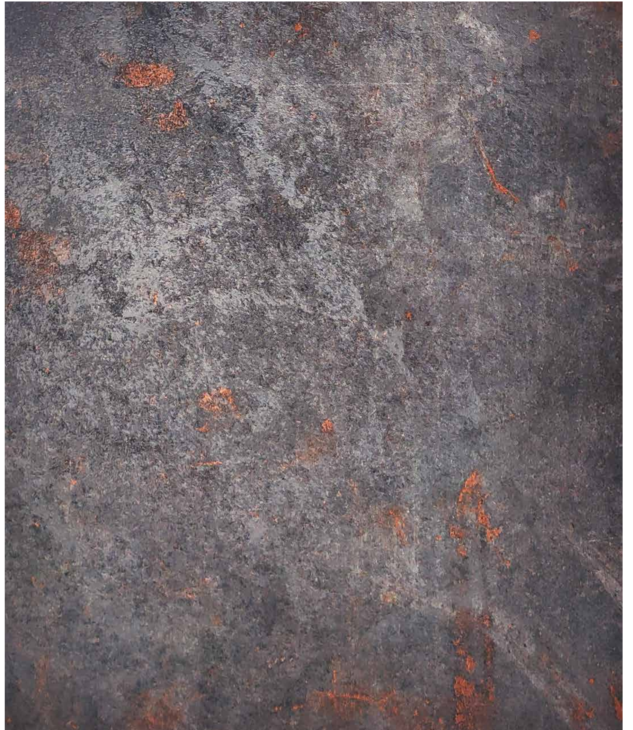
1006 RT | DARK-ICE
