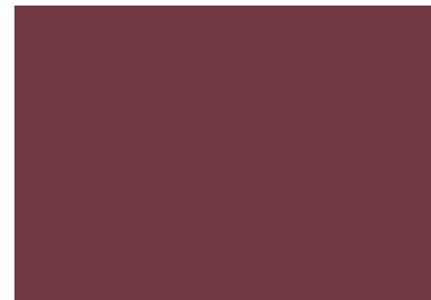
1194 SG | CRANBERRY
