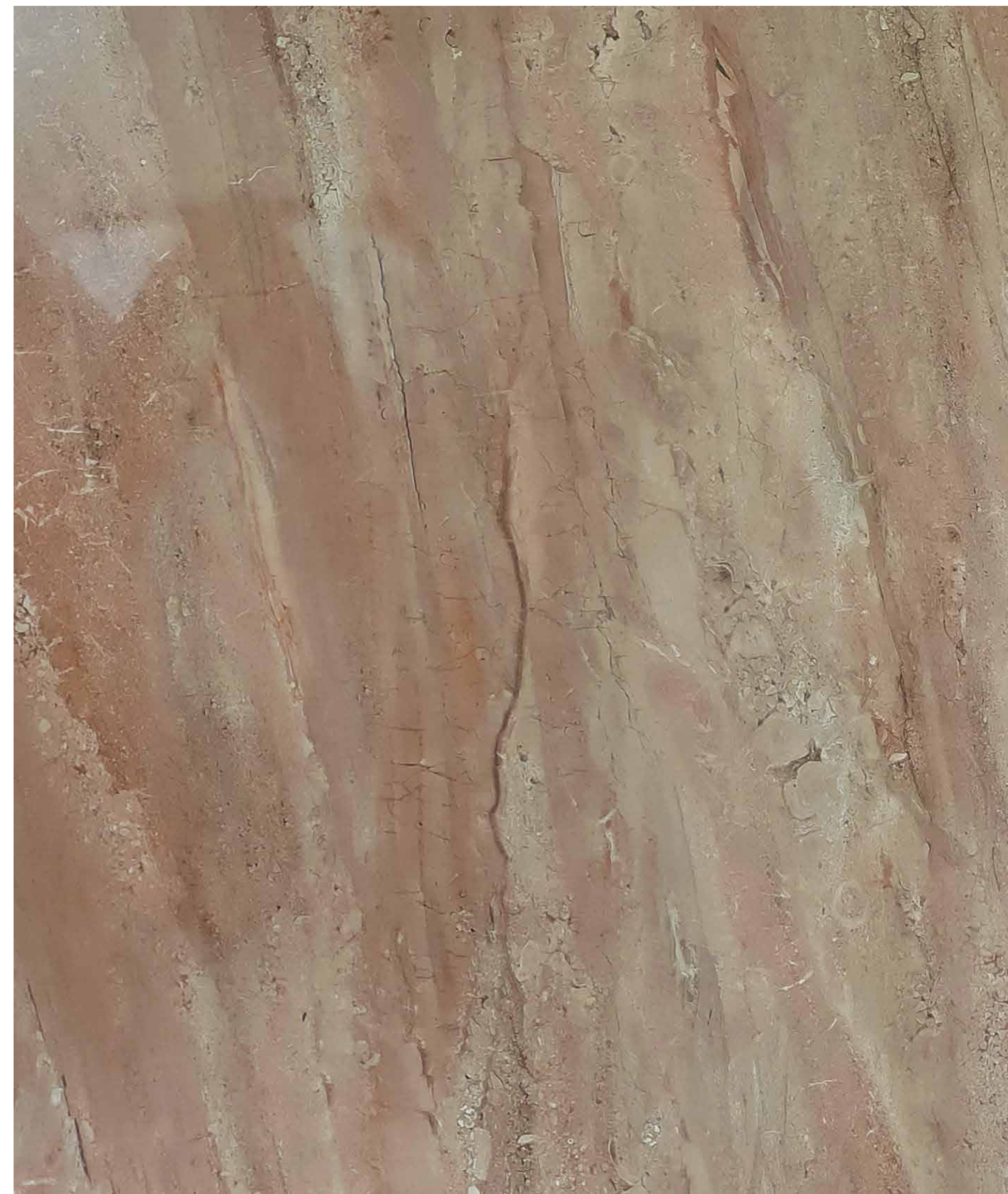
1305 SG | MASTERPIECE
