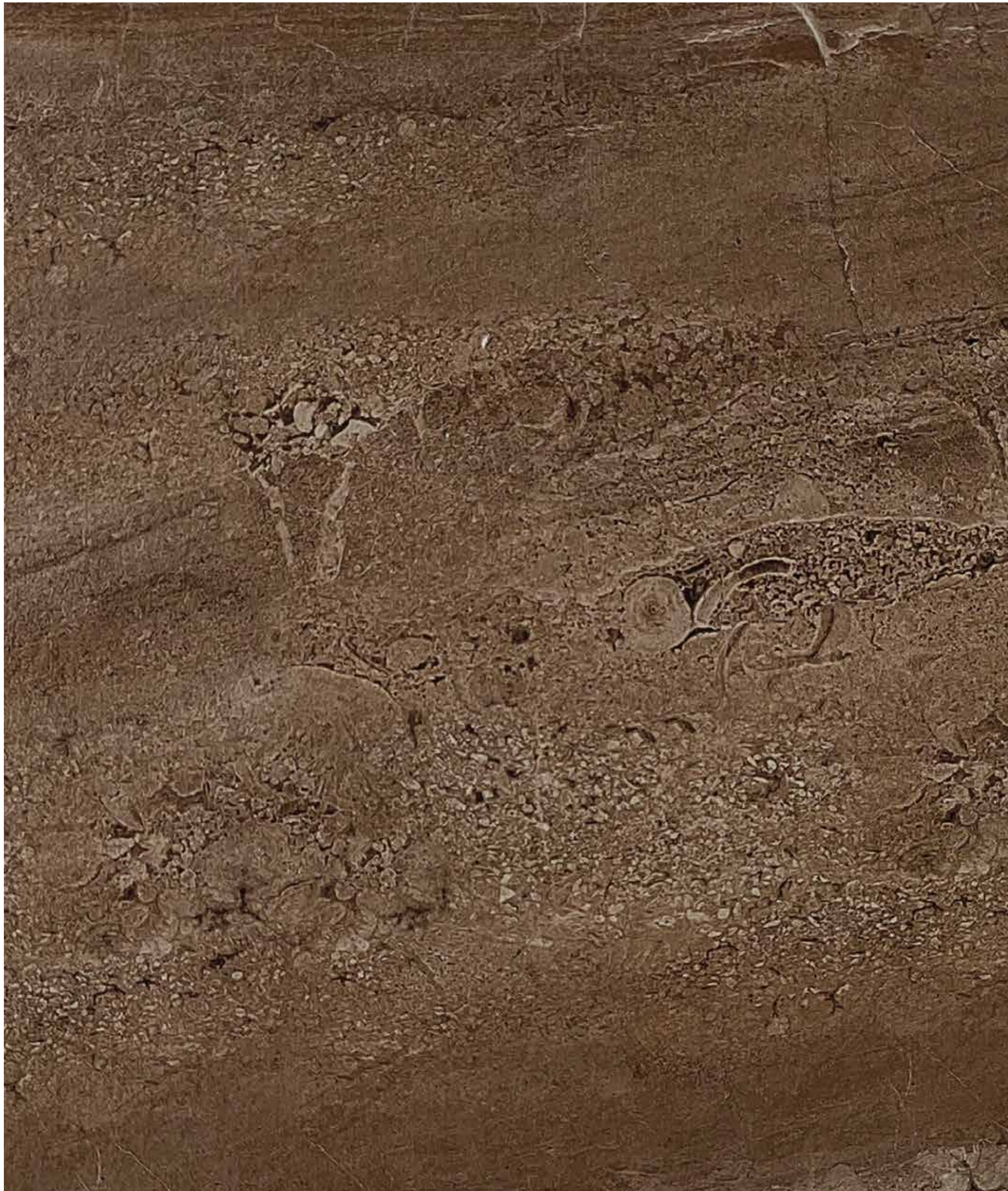
1305 MM | MASTERPIECE
