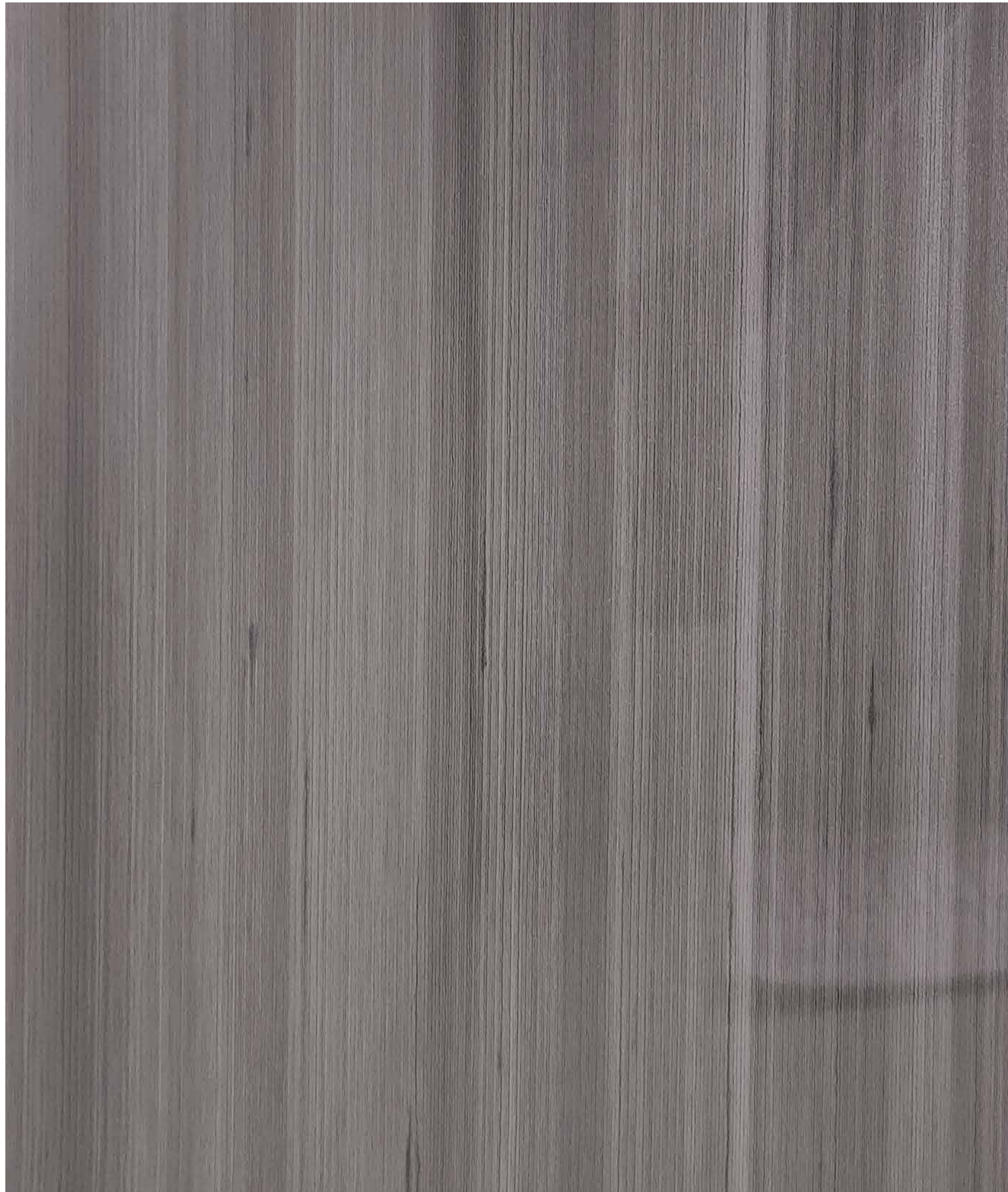
1009 SG | ASHBURY
